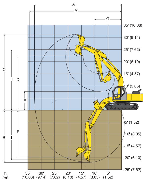
This chart is a graphic representation of the working ranges for the SK210LC equipped with a 9'8" (2.94 m) arm.
